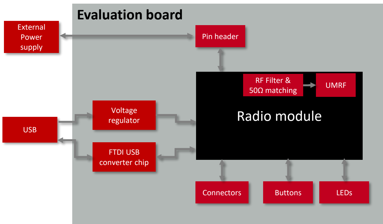
Figure 3: Block diagram
